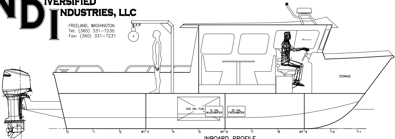
INBOARD PROFILE
