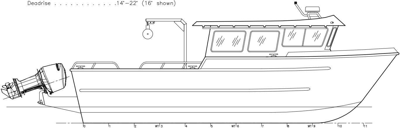
OUTBOARD PROFILE
