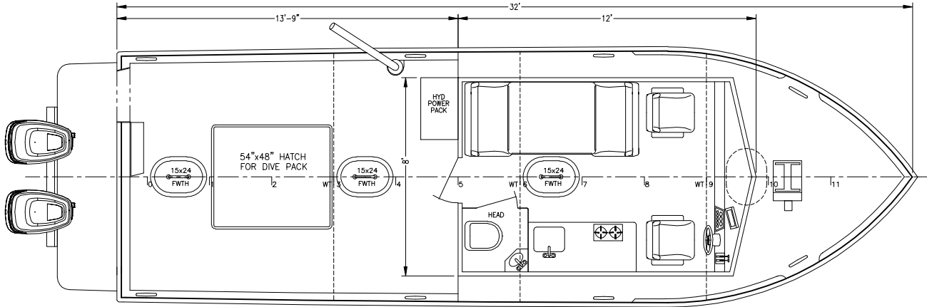
MAIN DECK ARRANGEMENT
