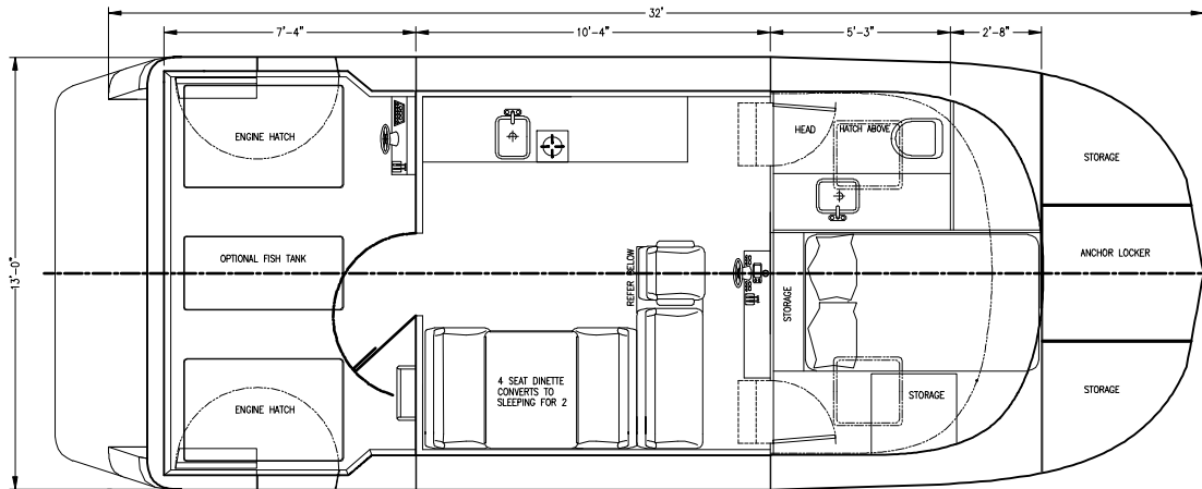
MAIN DECK
