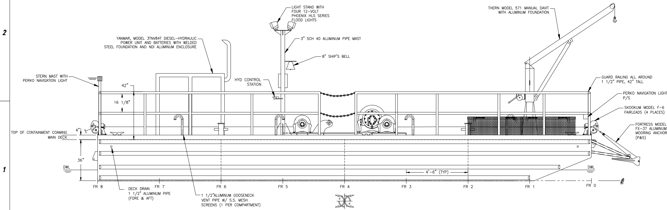
ELEVATION 1-4A OUTBOARD PROFILE SCALE: 1/2"=1'-0"
