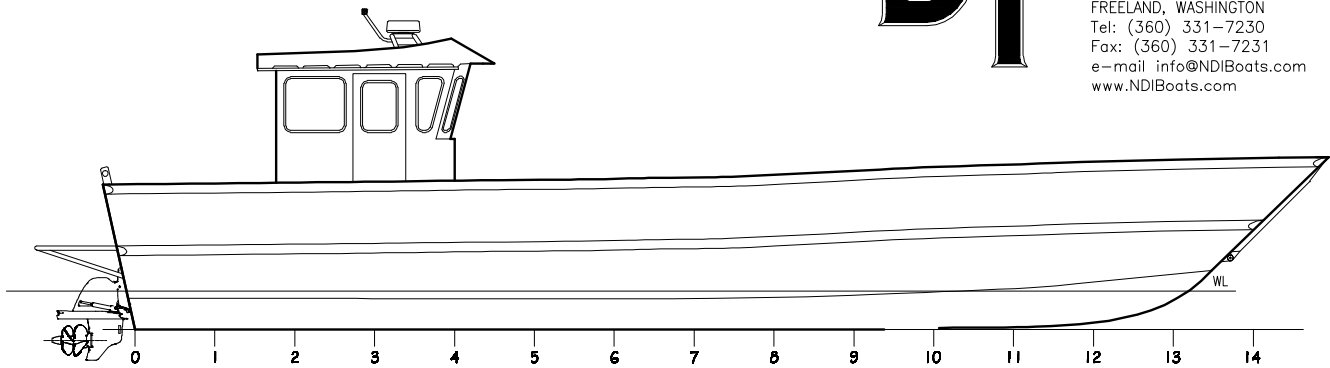
OUTBD PROFILE
