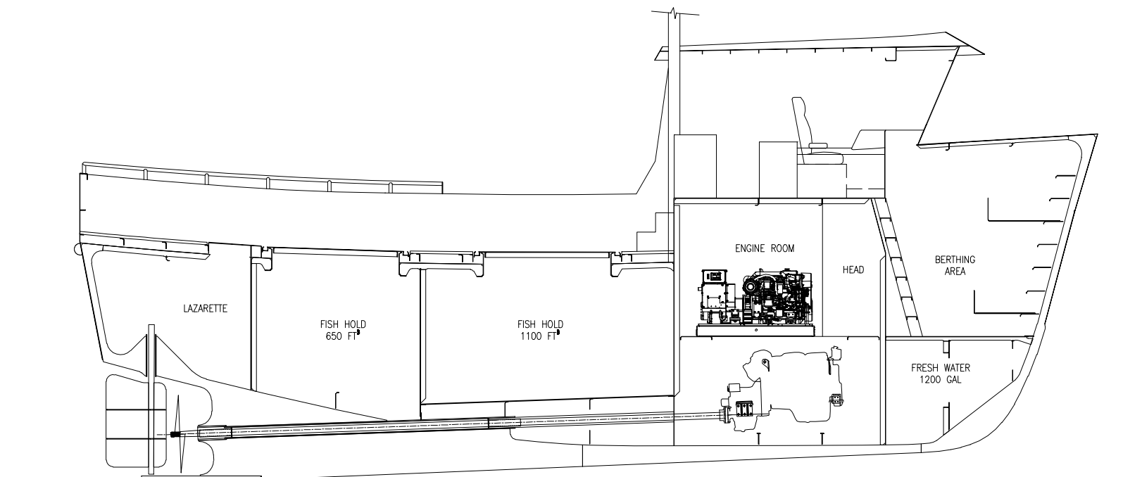
INBOARD PROFILE
