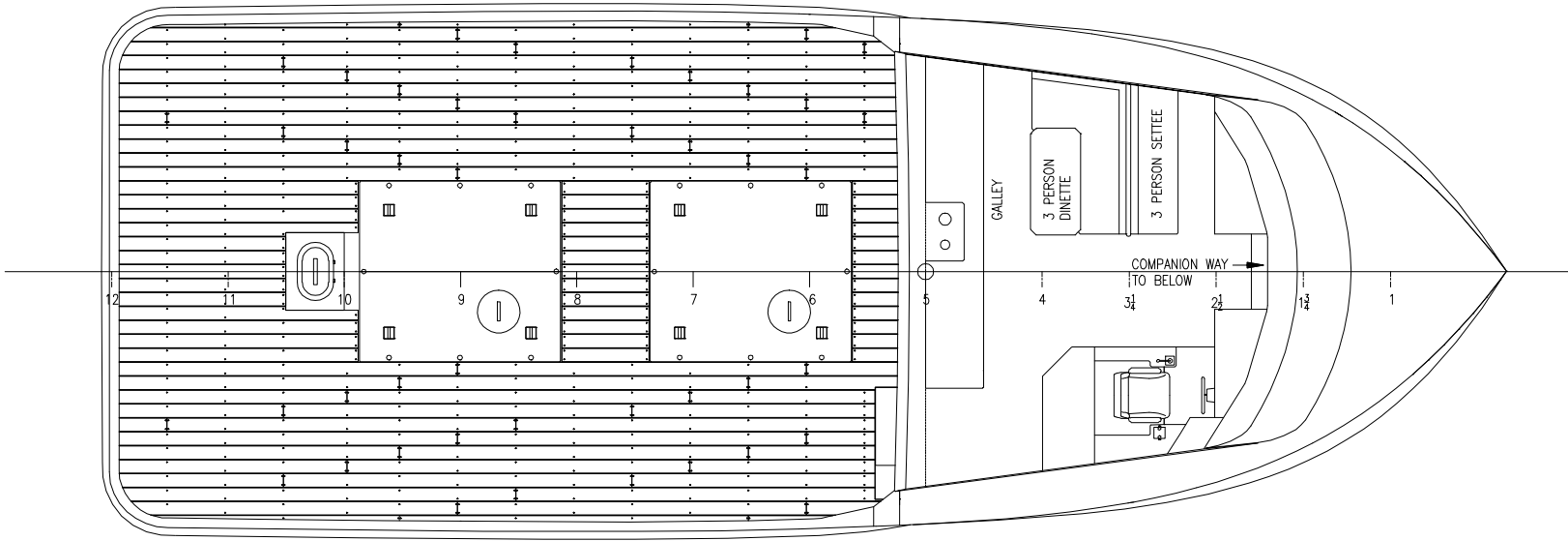
MAINDECK PLAN
