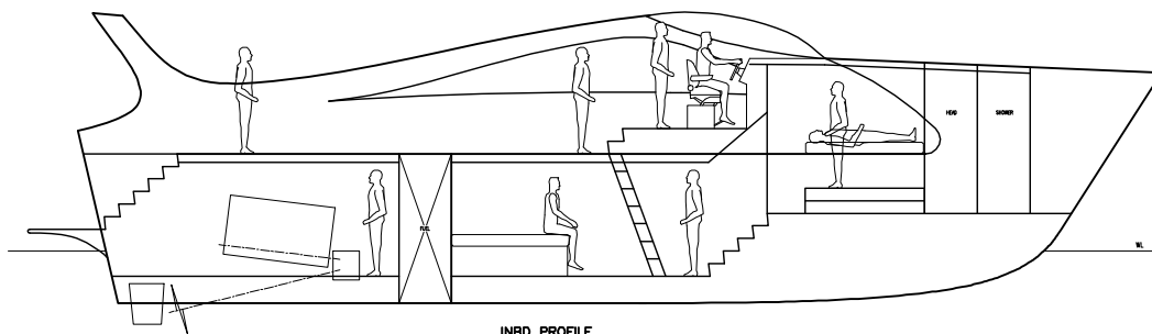
INBD PROFILE
