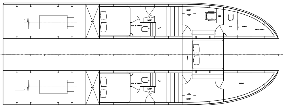
BELOW DECK PLAN
